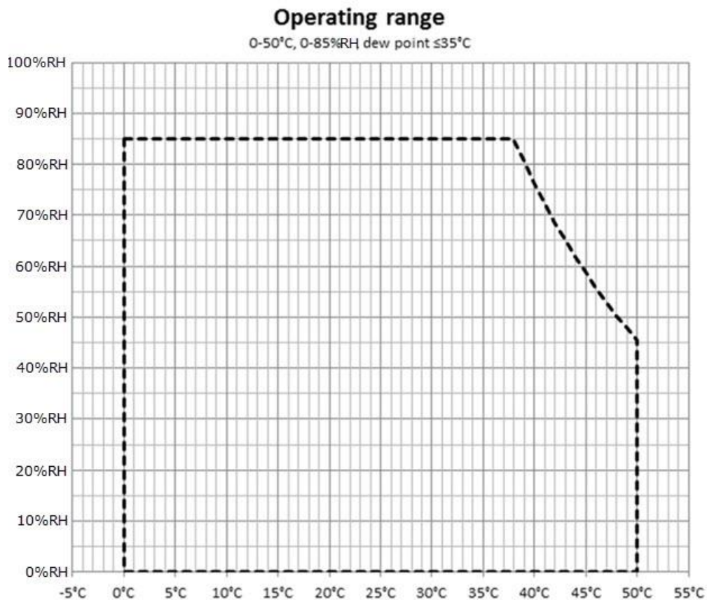
Figure 3 Operating range
