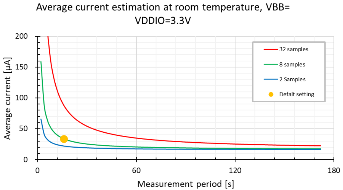
Figure 4 Average current
