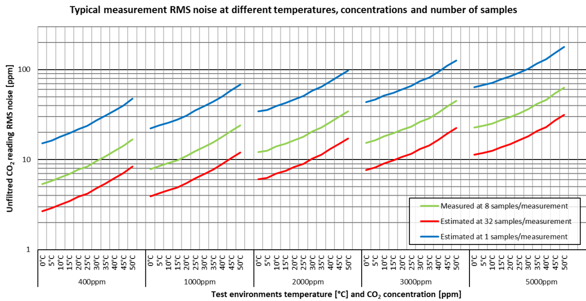
Figure 5 Measurement RMS noise
